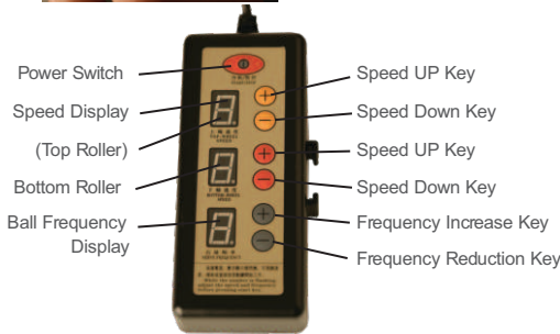
SPEED MODULATION ADJUSTMENT OF SPEED
